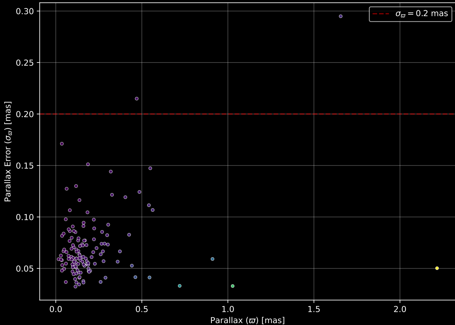
APOGEE DR17 Field: [002-05-O] Parallax Quality (n= 132)
