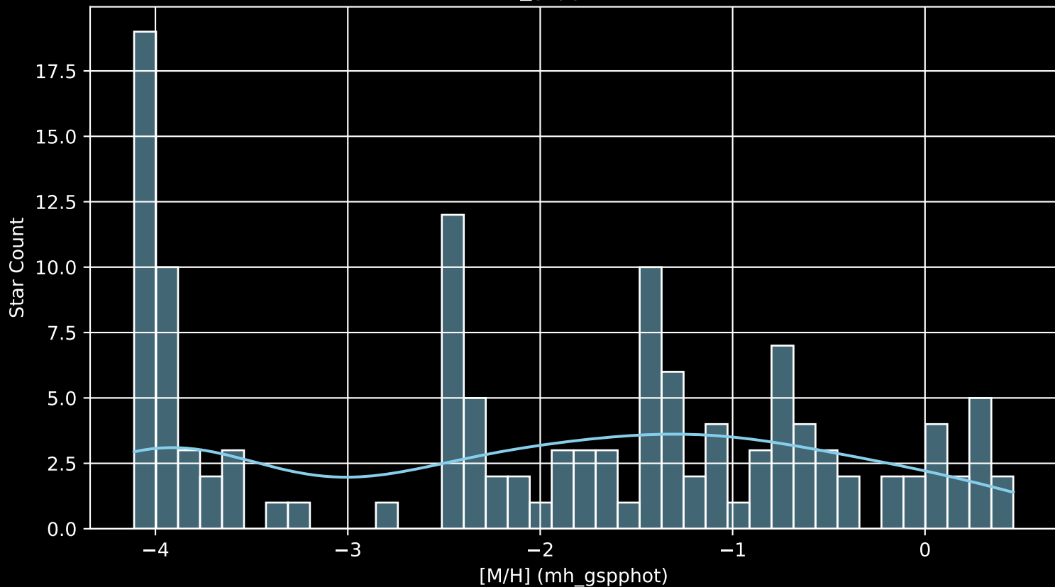
APOGEE DR17 Field: [002-05-O] [M/H] (mh_gspphot) (n= 131)
