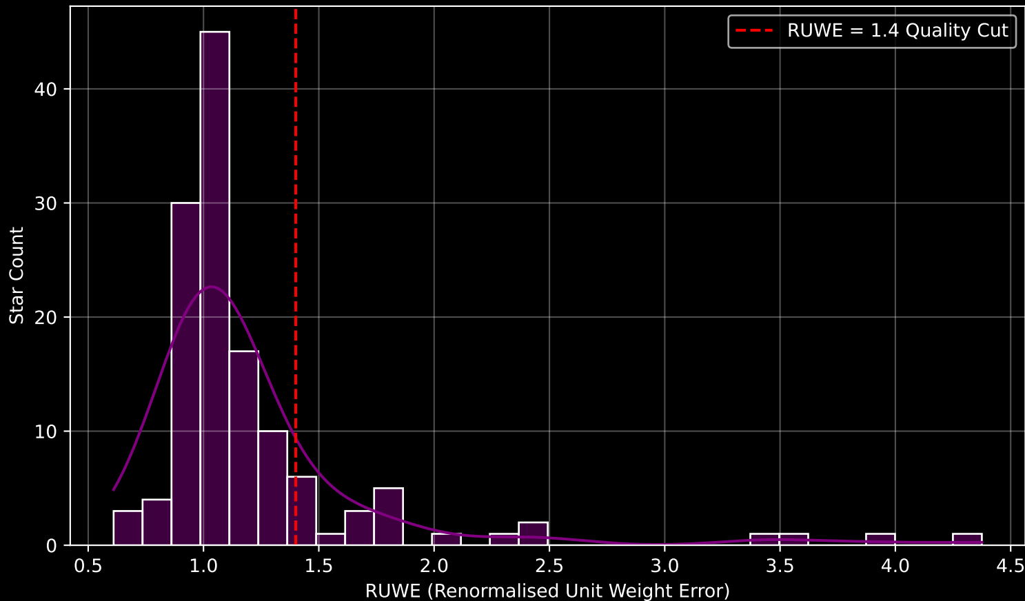
GAPOGEE DR17 Field [002-05-O] RUWE Distribution (n= 132)
