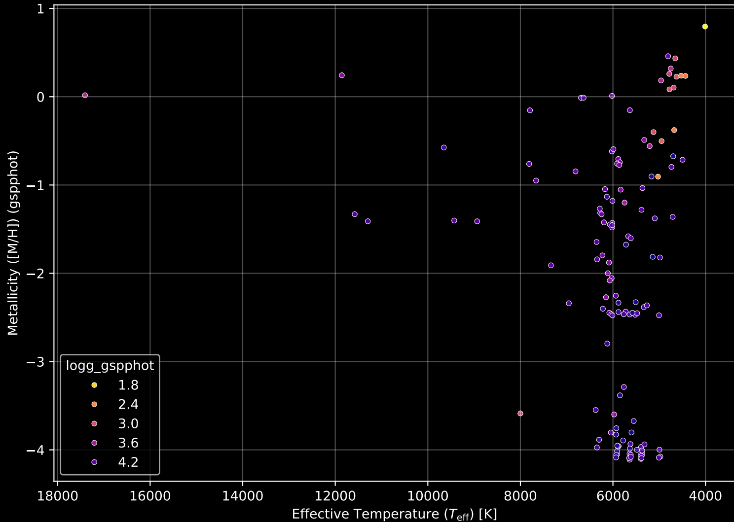
APOGEE DR17 Field: [002-05-O] Stellar Population Parameters (n= 132)
