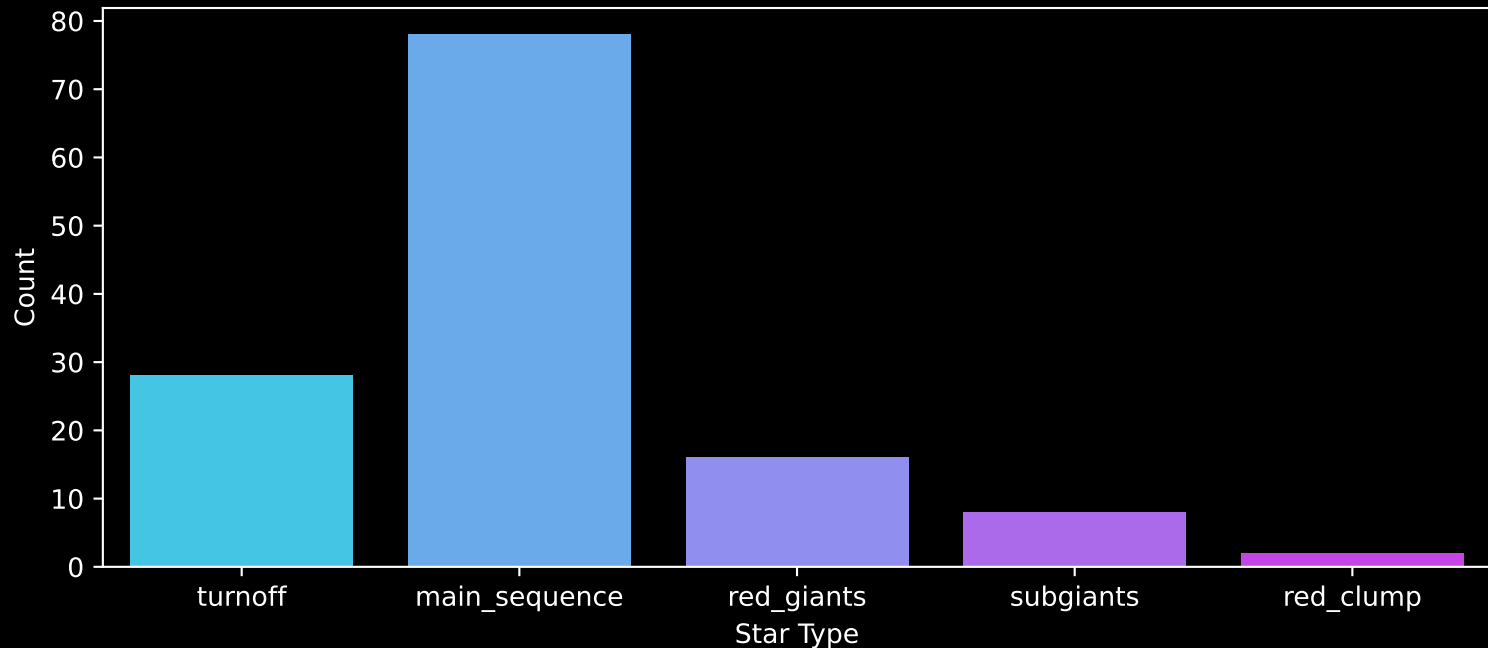
APOGEE DR17 Field: [002-05-O] Count plot of Star Type
