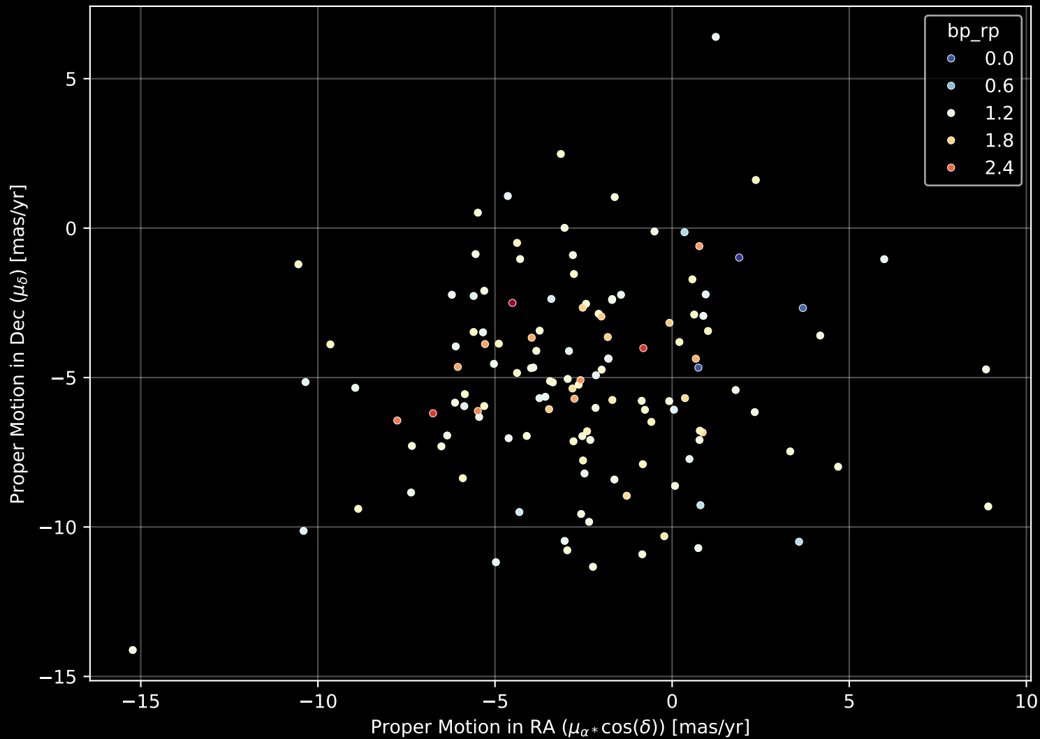
APOGEE DR17 Field: [002-05-O] Proper Motion Diagram (n= 132)
